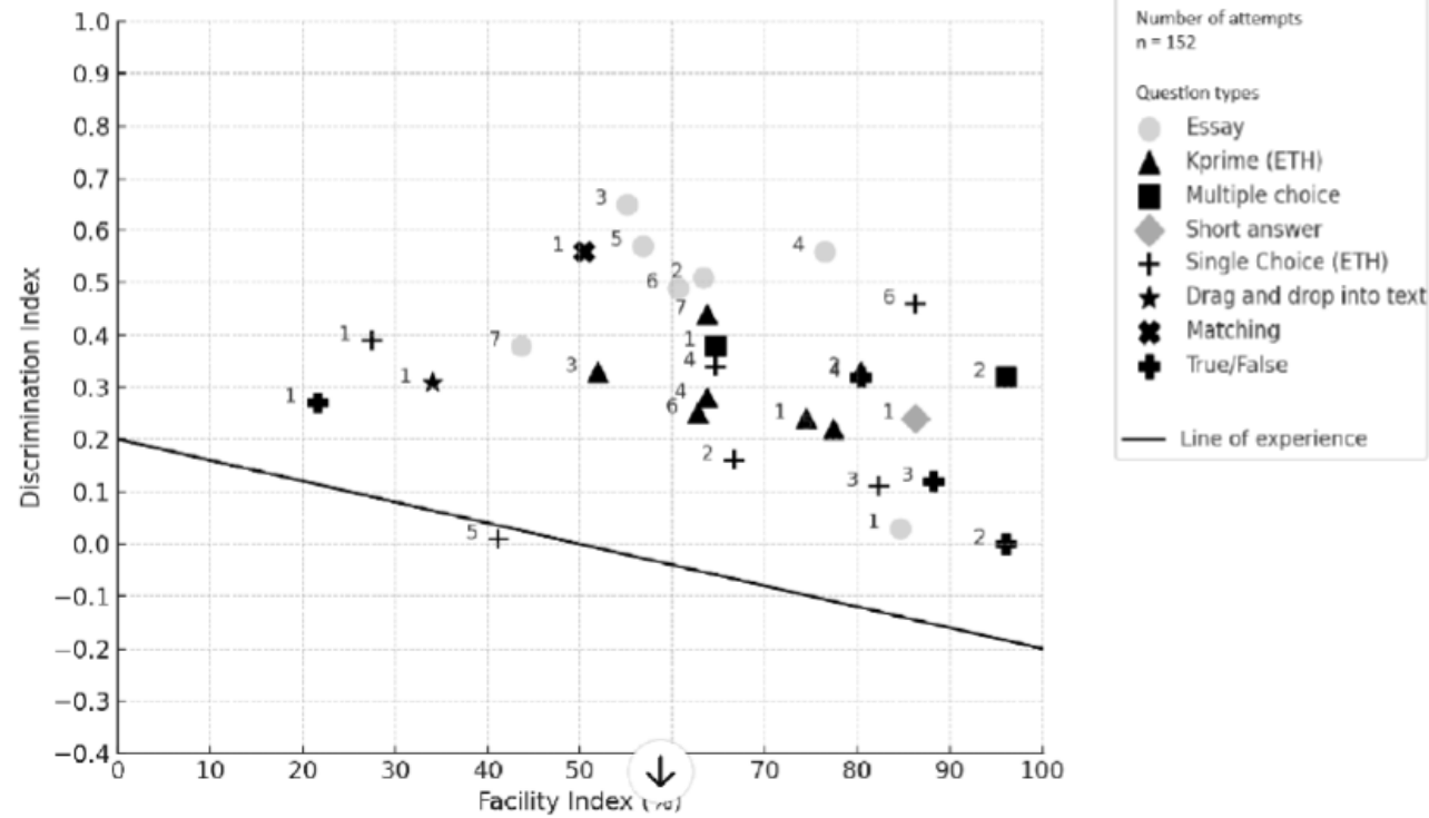
Scatter plot of questions: Facility index vs. discrimination index
